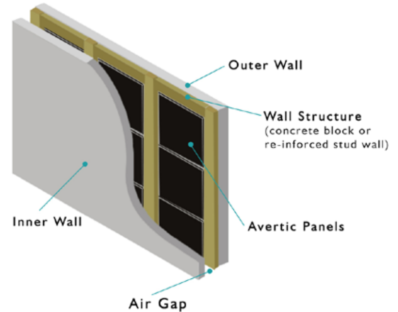
Example of secure room wall construction
